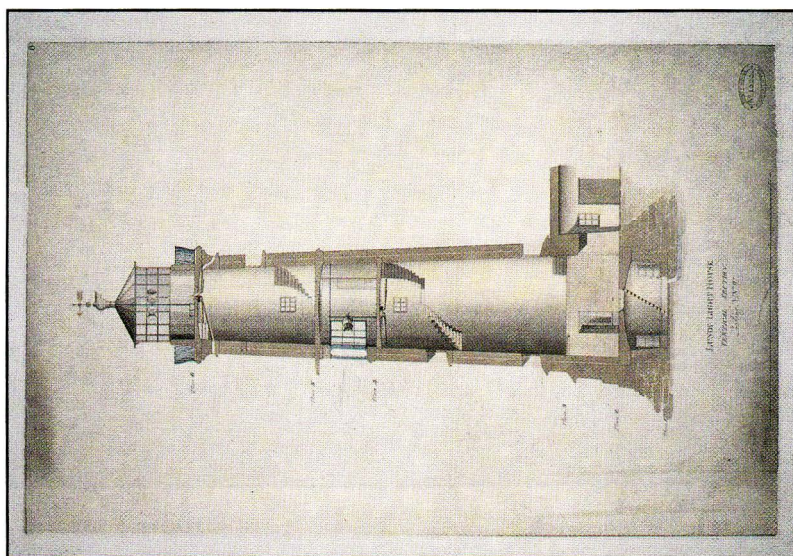
Plate 6: Lundy Lighthouse, vertical section (1322). From Farrah's paper.
