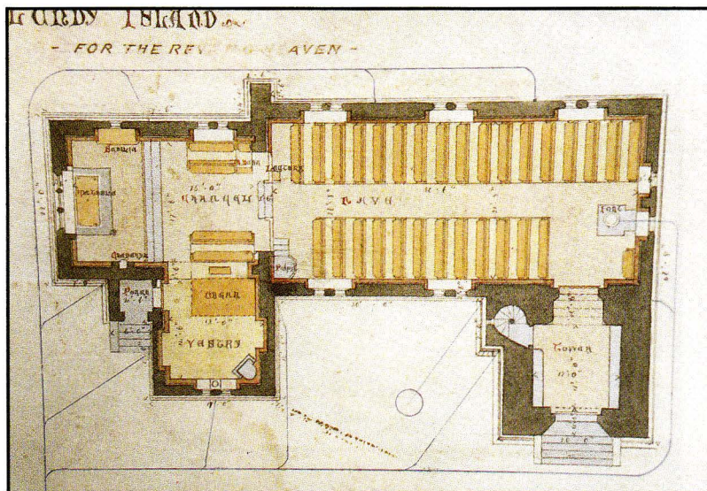
Plate 1: Copy of the architect's plan of St. Helena's Church, Lundy (from Farrah's paper) (Photo: Lorna Gibson)
